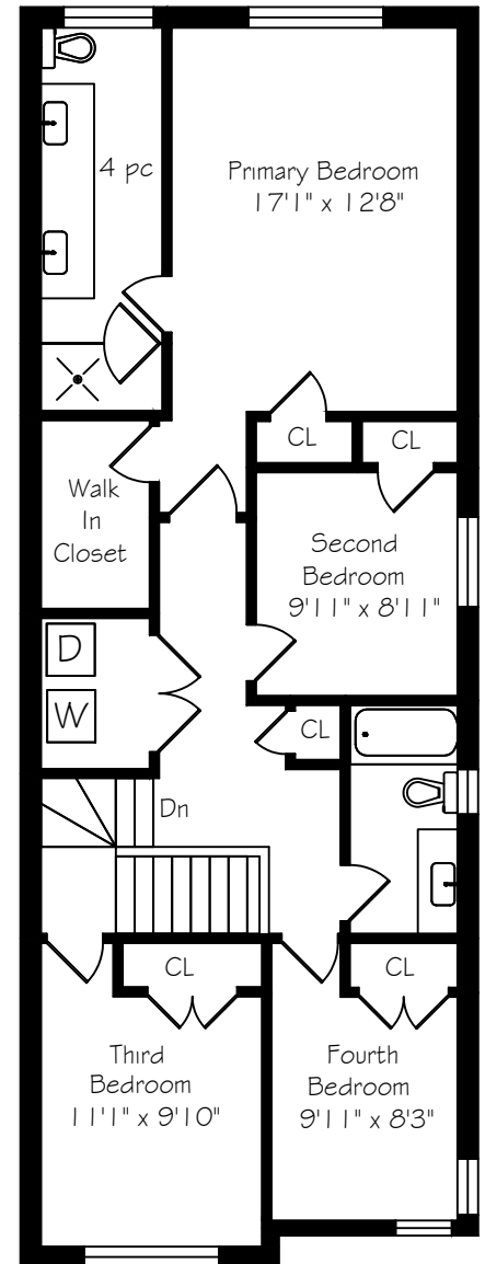
Second Floor 1098 Square Feet
