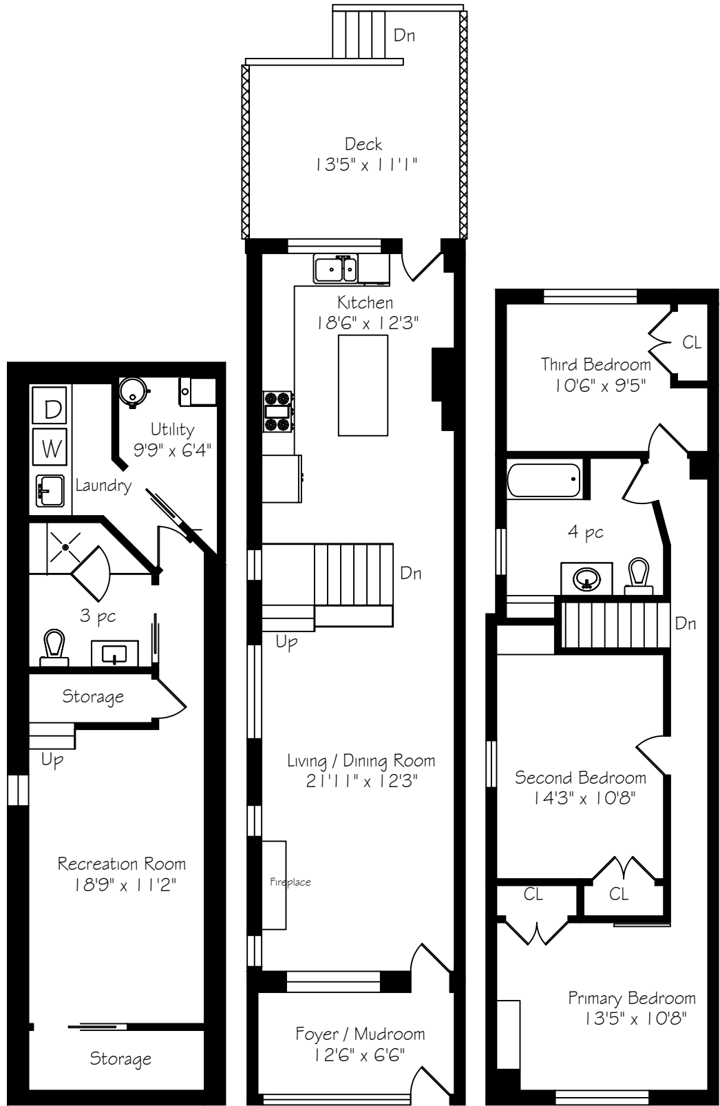
Lower Level 632 Square Feet
