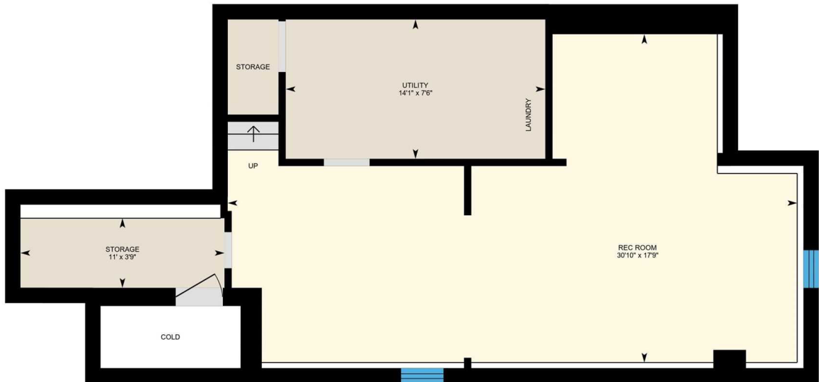
BASEMENT
