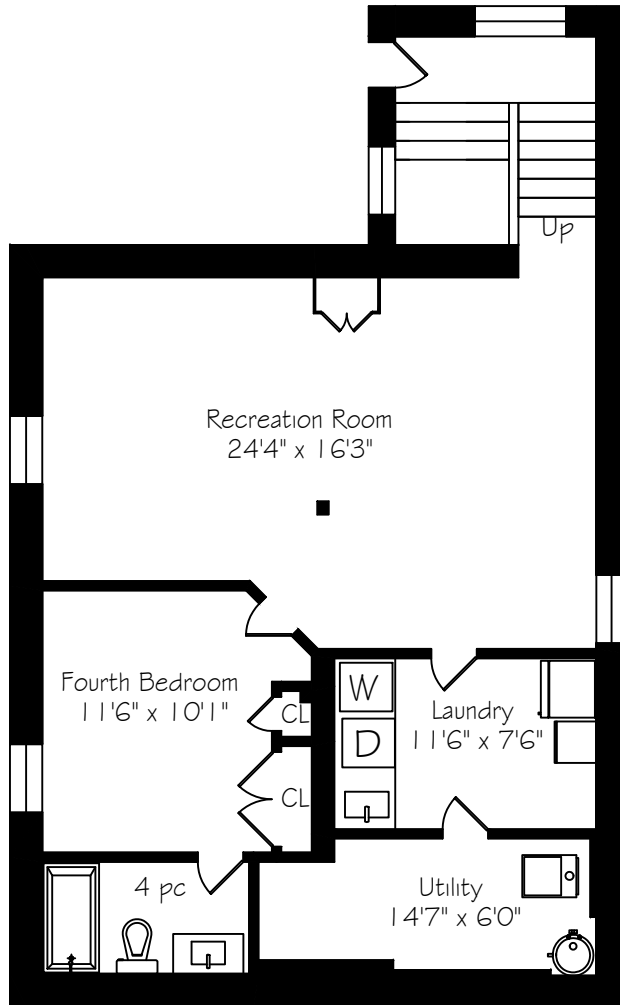
Lower Level 1024 Square Feet
