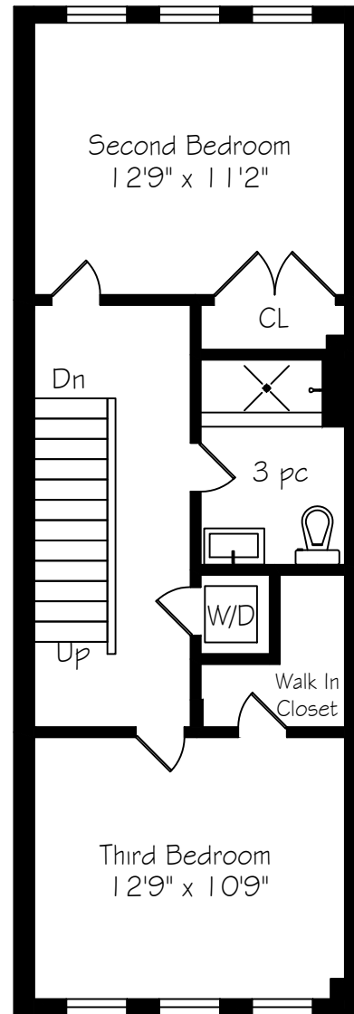
Second Floor 580 Square Feet
