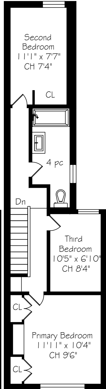
Second Floor 572 Square Feet
