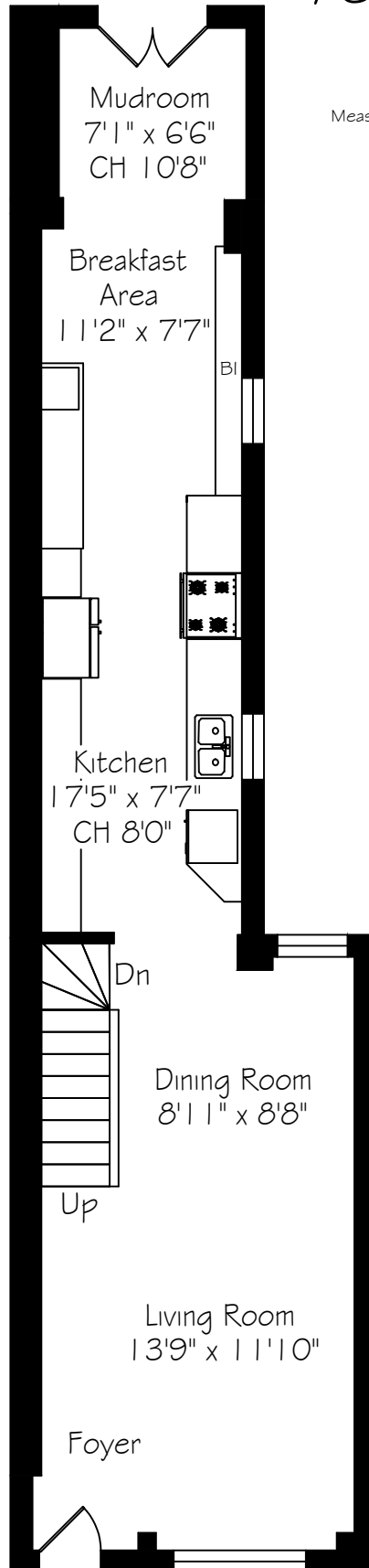
Main Floor 630 Square Feet
