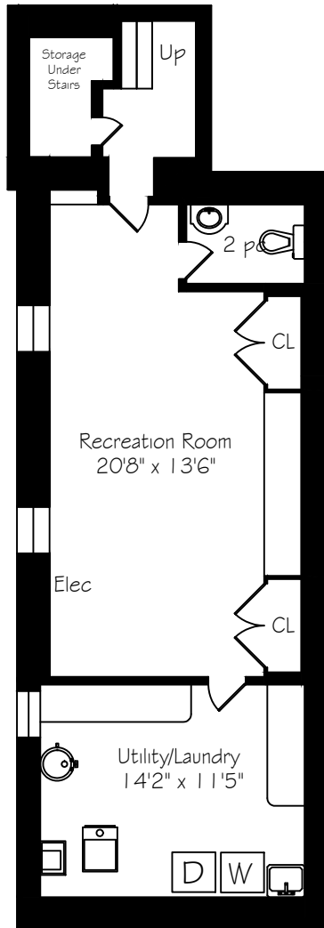
Lower Level 754 Square Feet
