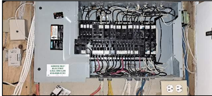
Breakers - basement
