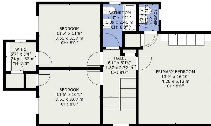
SECOND FLOOR
